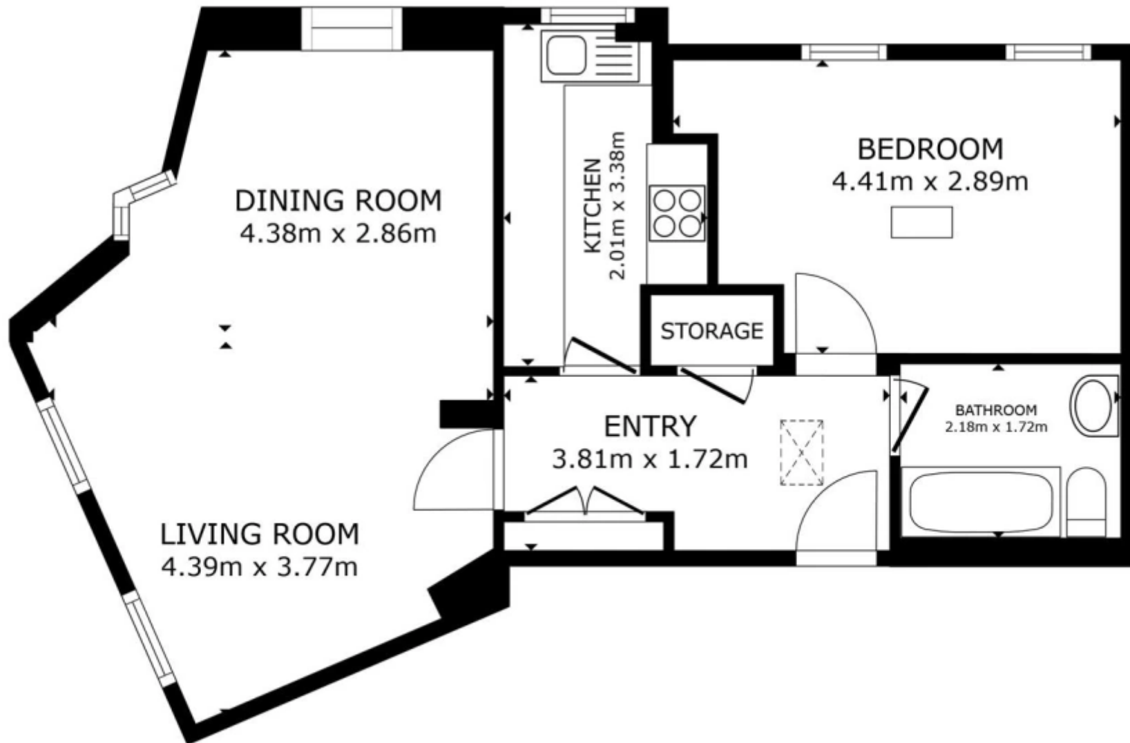
FLOOR PLAN
